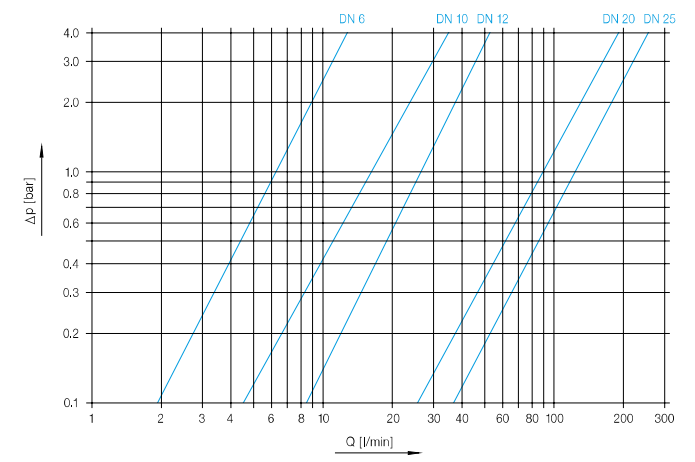
Multi-way ball valves with trunnion ball for manifold mounting with L-bore
