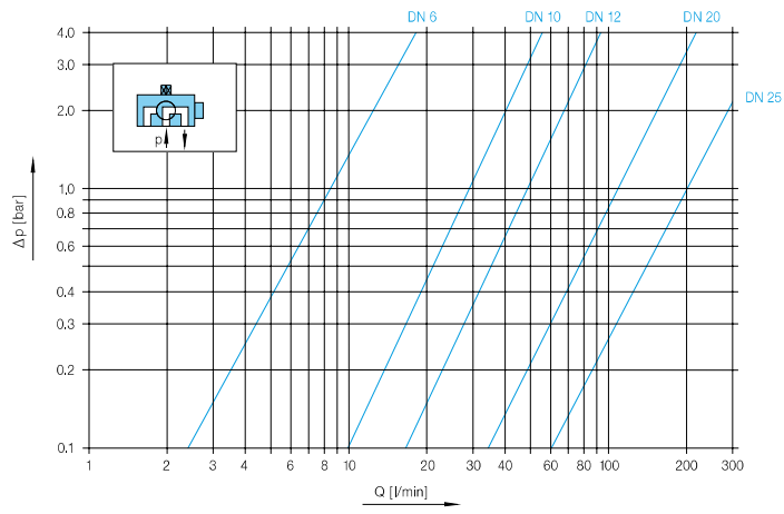
Multi-way ball valves with floating ball for manifold mounting with L-bore
