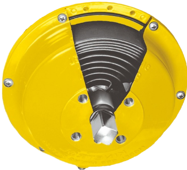
Spring housing cut away
